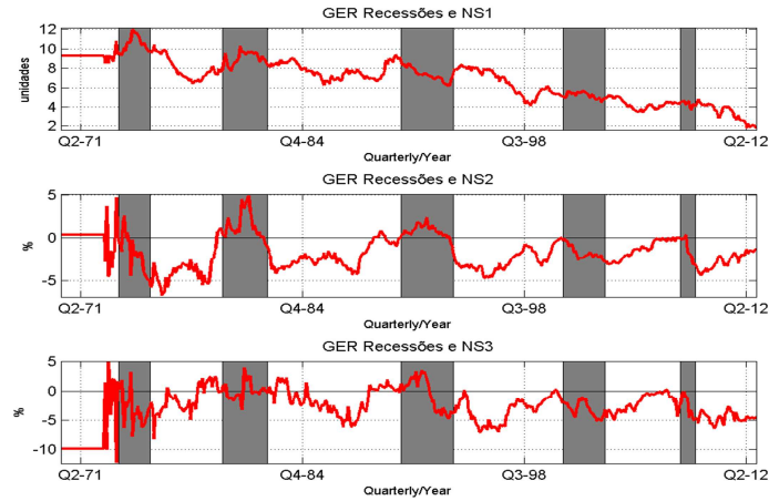
Figure 1: Germany Recessions and yield curve components estimated evolution
