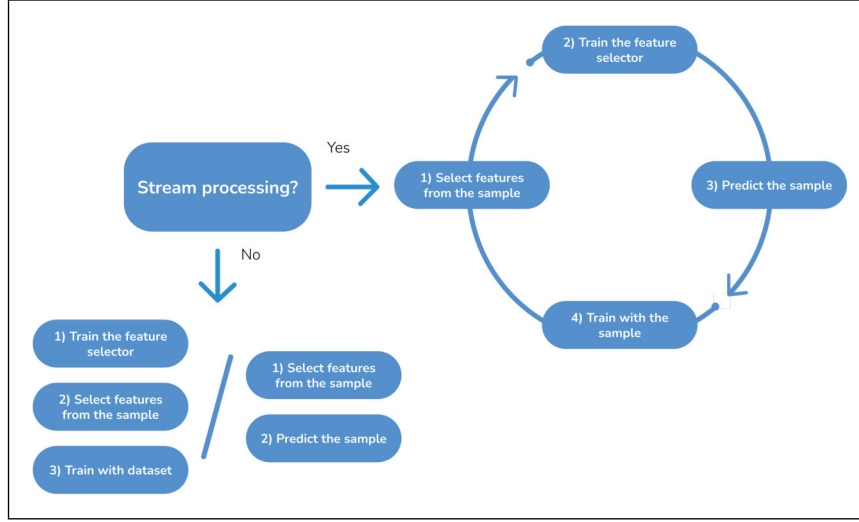
Figure 2. Streaming and batch supervised learning.
